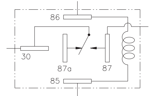
Horn Relay
